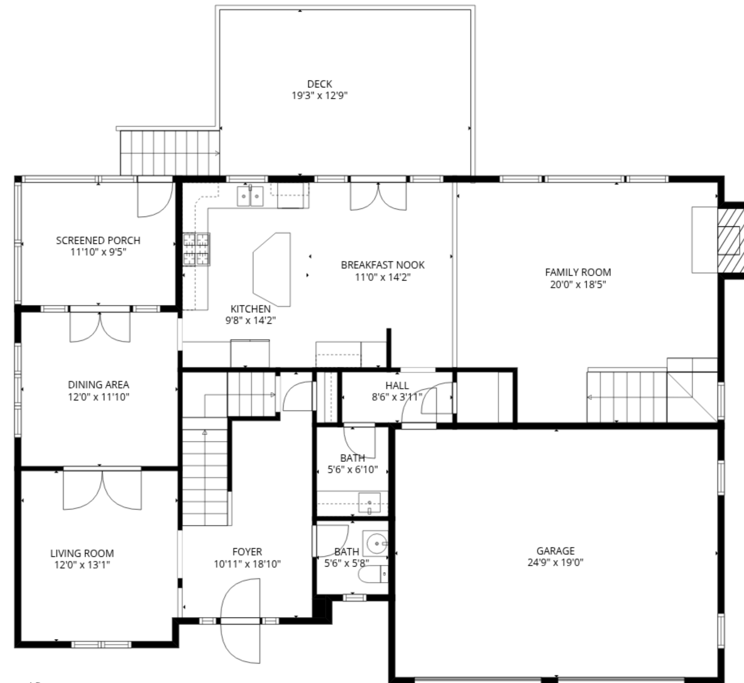
2nd floor
